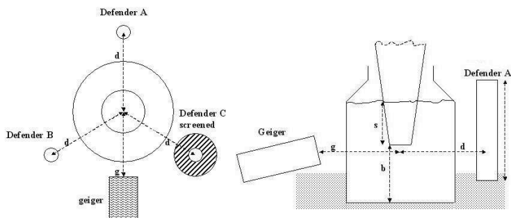
Fig. 2: Layout and lateral section of the experimental setup. d=7 cm, g=10 cm, s=4 cm, b=5 cm. This setup indicates that between the cavitation area and the neutron detectors and the Geiger counter there were 3.5 cm of water, the thickness of the Borosilicate (about 2 mm) and few centimetres of air.
