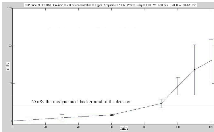
Fig. 4: Neutron dose (nSv) vs. cavitation time for \text{Fe}(\text{NO}_3)_3 solution. The horizontal line represents the background level.
