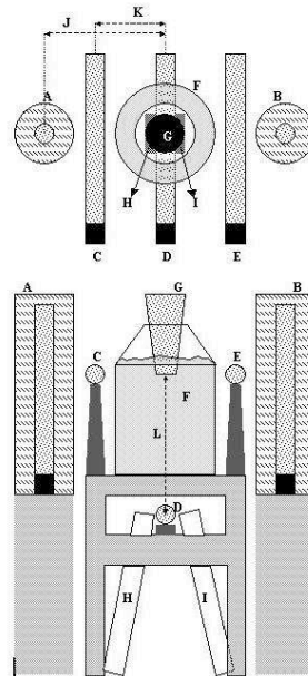
Fig. 5: Experimental apparatus used in the second investigation. The cavitation Chamber (F) is visible in the middle of both pictures and the sonotrode, the vertical tapered metal stick (G), is aligned with and inserted in it. The green pipe surrounding the sonotrode conveyed the cooling air onto the sonotrode surface. The three horizontal greyish cylinders (C,D,E) with a black cylindrical endcap are the neutron detectors. The two orange (right) (B) and creamy (left) (A) vertical cylinders contained the two screened Defenders, one by boron (orange) and the other by carbon (creamy).
