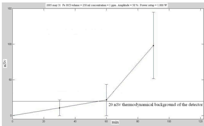
Fig. 3: Neutron dose (nSv) vs. cavitation time for \text{Fe}(\text{Cl})_3 solution. The horizontal line represents the background level.
