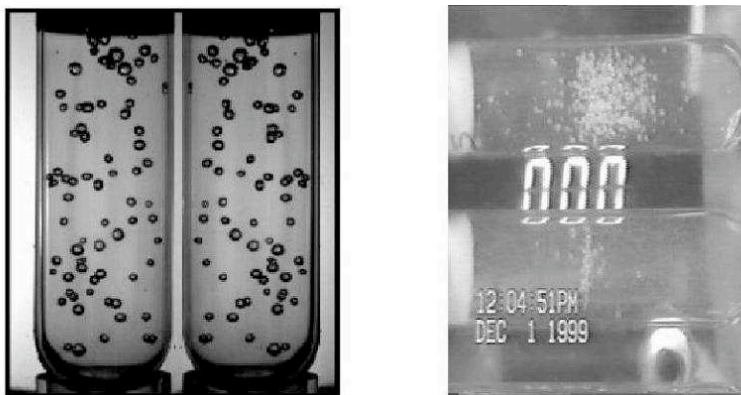
Fig. 1: Morphology and distribution of bubbles produced in a Defender by the passage of neutrons (left); heavy ions (right). In the second picture, the ion beam goes from bottom to top.
