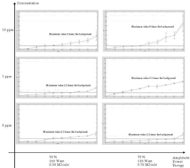
Fig. 6: The six graphs (one for each cavitation of the second series) showing the neutron dose (in nSv) as a function of time in minutes (time interval 10 min). Each curve corresponds to one value of concentration and one of the amplitude. The horizontal line in all graphs corresponds to the thermodynamical noise of 3.5 nSv. The graphs are displaced in a Cartesian plane, with concentration (in ppm) on the y-axis and amplitude (power) on the x-axis.
